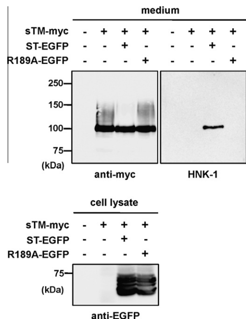
Fig. 2. Requirement of the sulfotransferase activity of HNK-1ST for the suppression of CS chain on TM. sTM-myc was co-transfected with ST-EGFP or the R189A mutant of HNK-1ST (R189A-EGFP). The secreted sTM-myc was pulled down and subjected to Western blotting using anti-myc and HNK-1 mAb (medium). The expression of HNK-1ST and HNK-1ST (R189A) was confirmed by Western blotting of the cell lysate (cell lysate).
